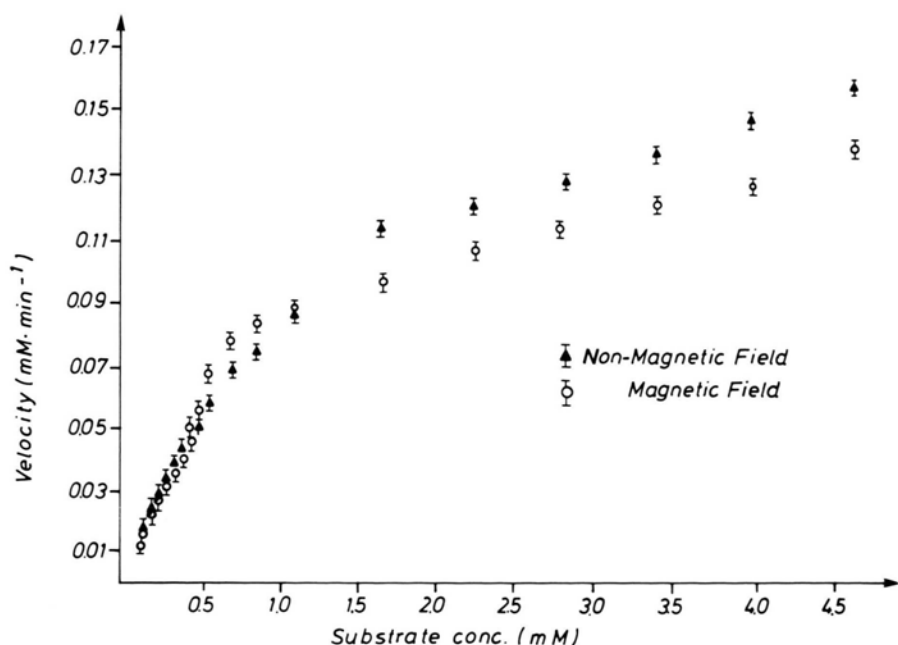
Fig. 1. The rate of oxidation of ascorbic acid by the enzyme is plotted vs. the concentration of the substrate. Each point – both control and sample exposed to 1.1 T magnetic field – represents the arithmetic mean of a triplicate experiment.
